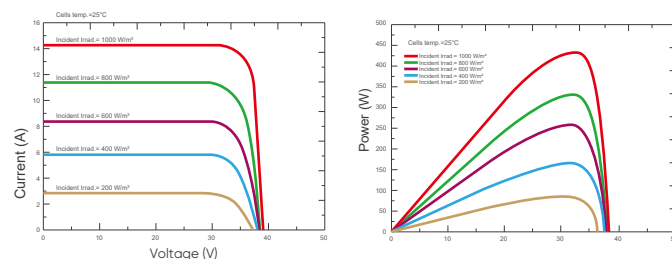
Current-Voltage & Power-Voltage Curves (RMHT54/430AB2)
